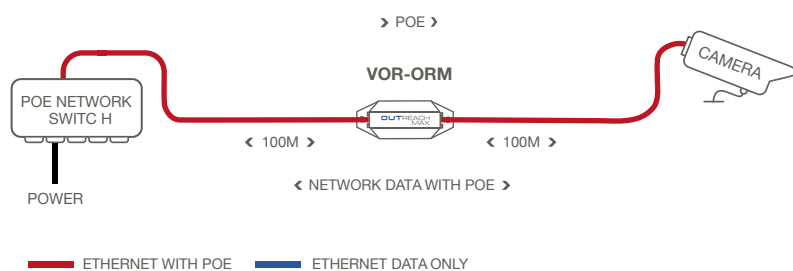
Diagram 1. A single OUTREACH Max doubles the cable range to a POE IP Camera. Each cable segment can be up to 100 metres.
