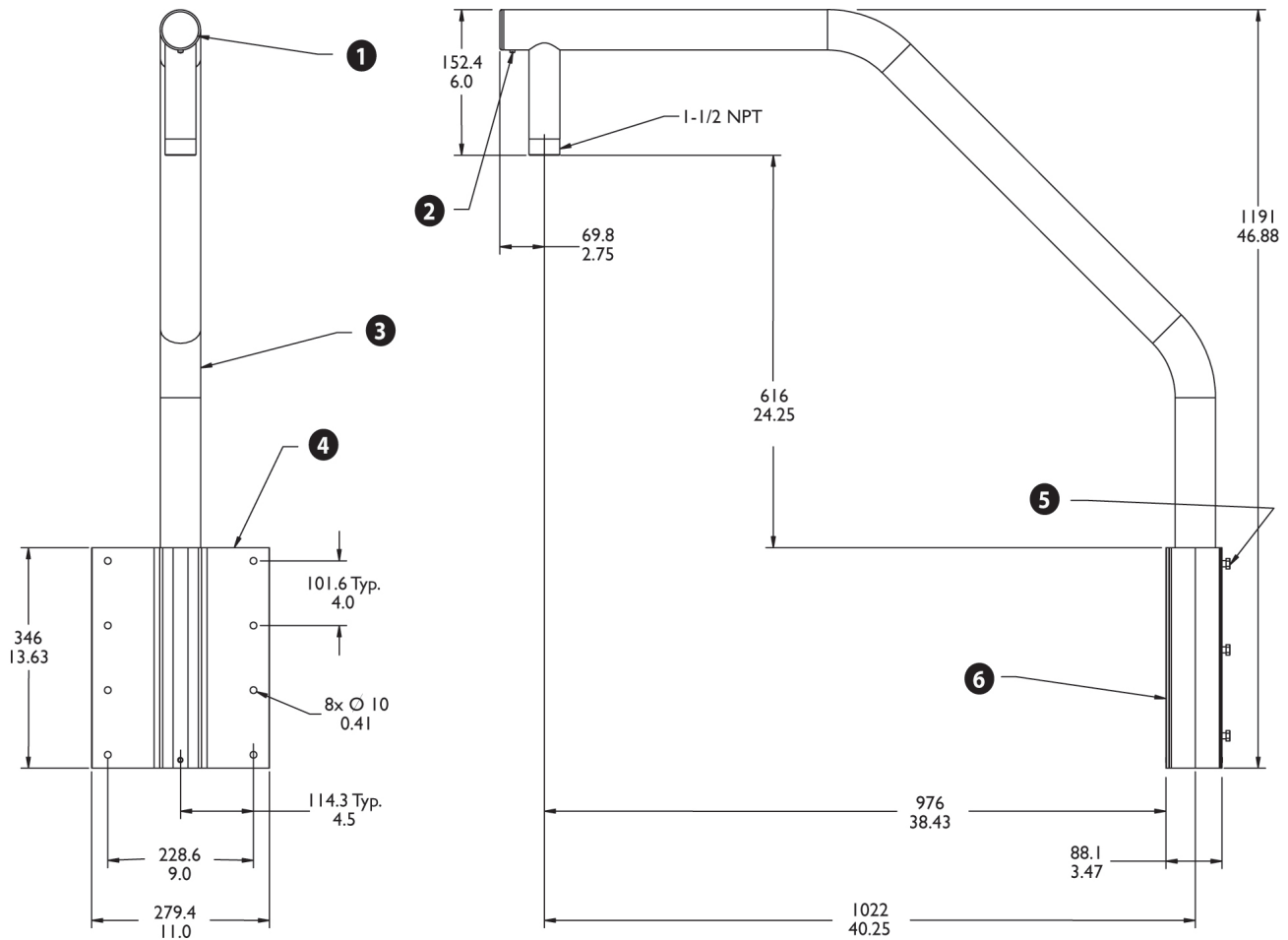
Figure 1: Dimensional Outline - LTC 9230/00 Parapet Mount (Shown with included wall mount bracket.)
