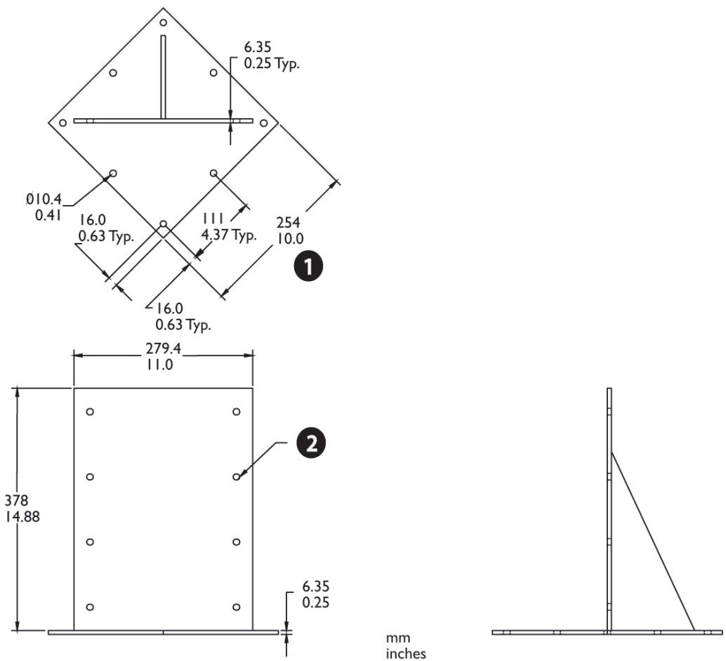
Figure 2: Optional LTC 9230/01 Roof Mount
